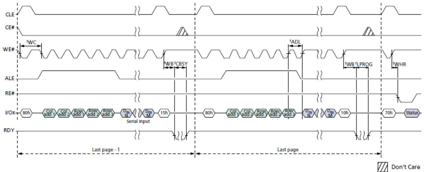
PROGRAM PAGE CACHE
