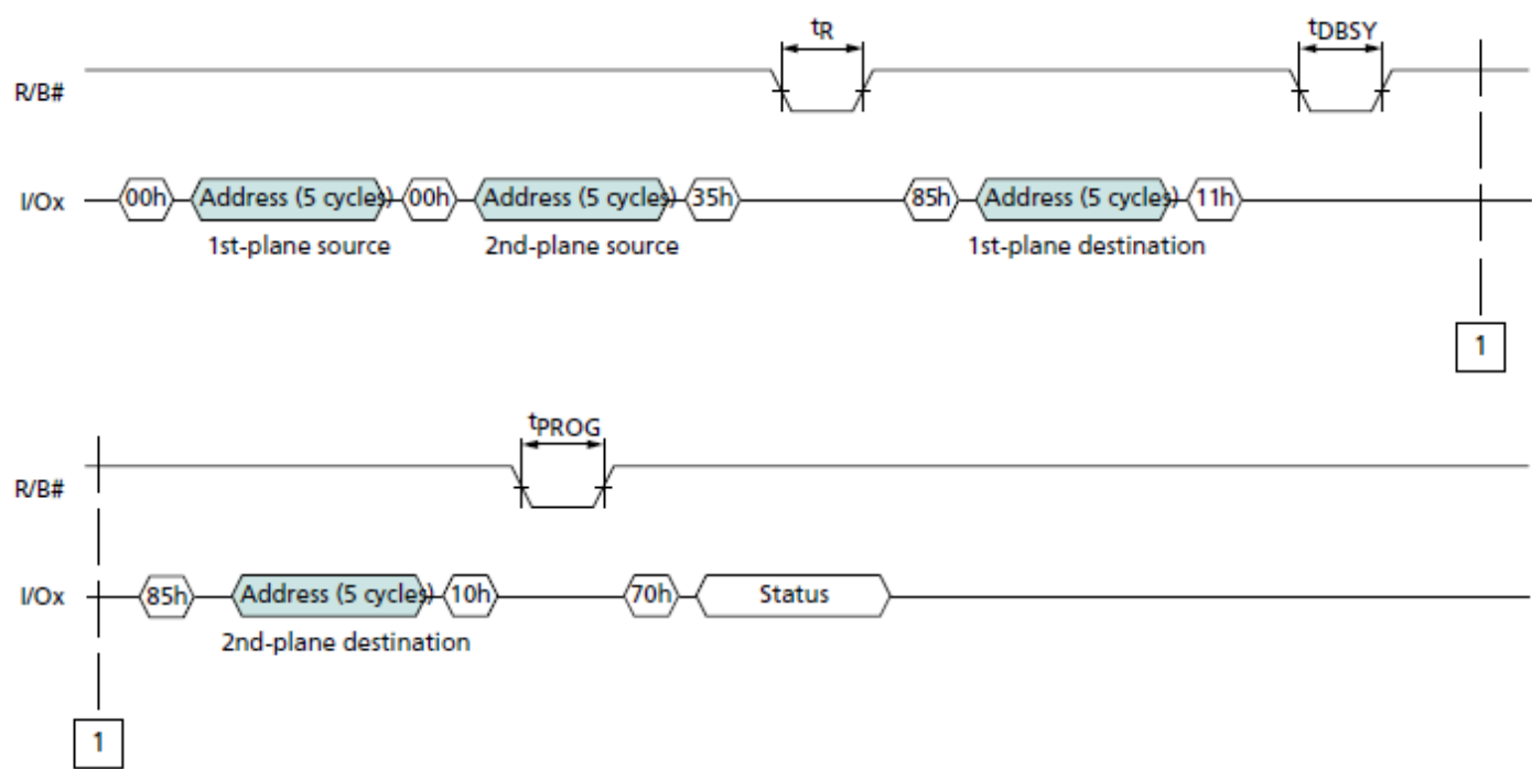
TWO-PLANE INTERNAL DATA MOVE
