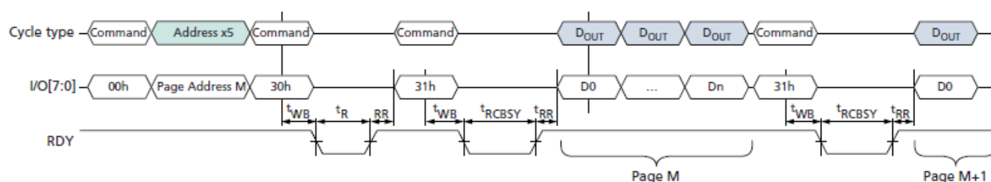
READ PAGE CACHE SEQUENTIAL (31h) Operation
