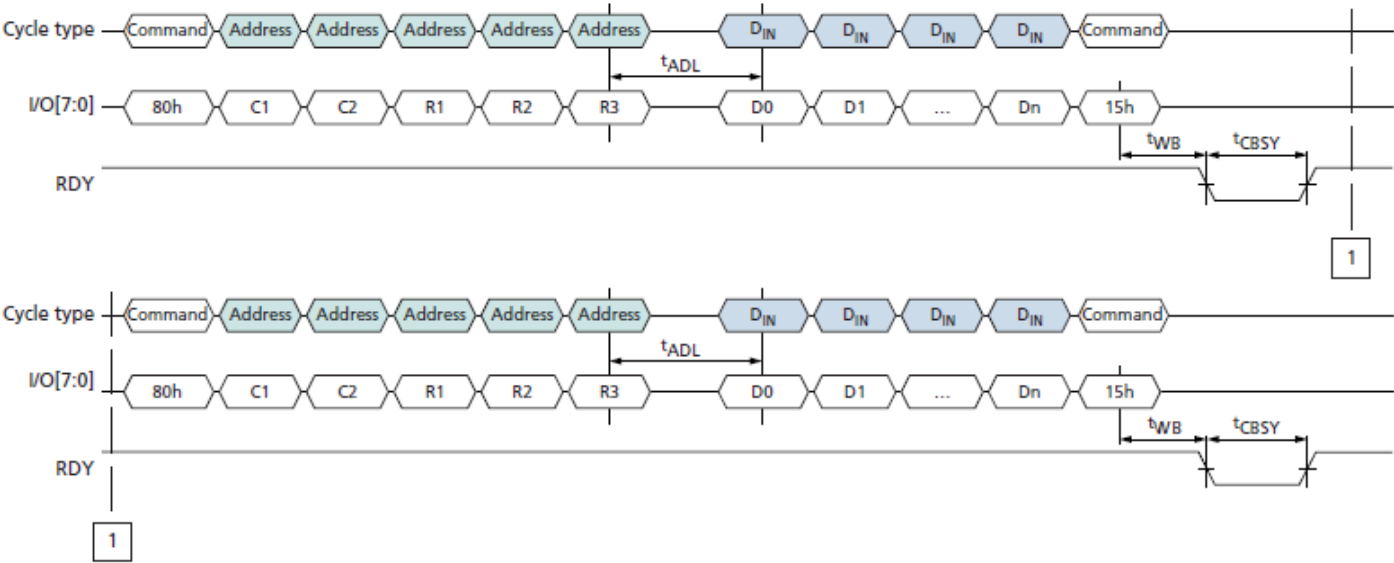
PROGRAM PAGE CACHE (80h-15h) Operation (Start)
