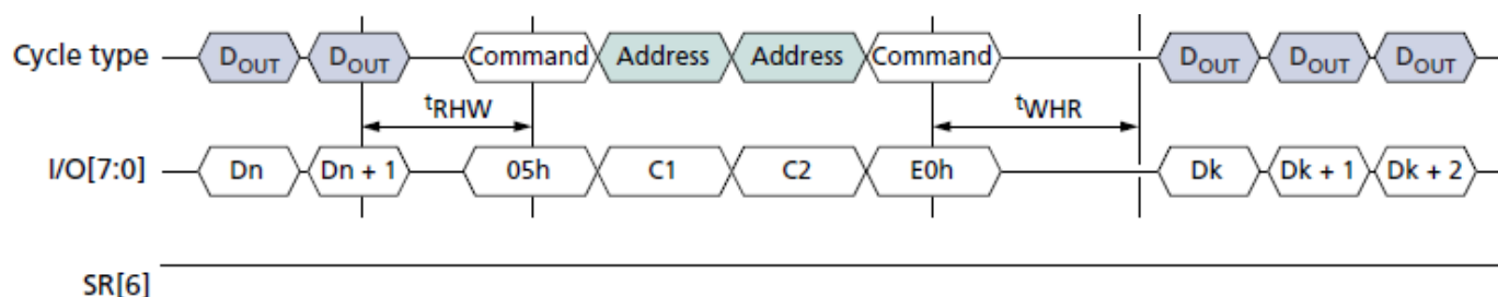
RANDOM DATA READ (05h-E0h) Operation
