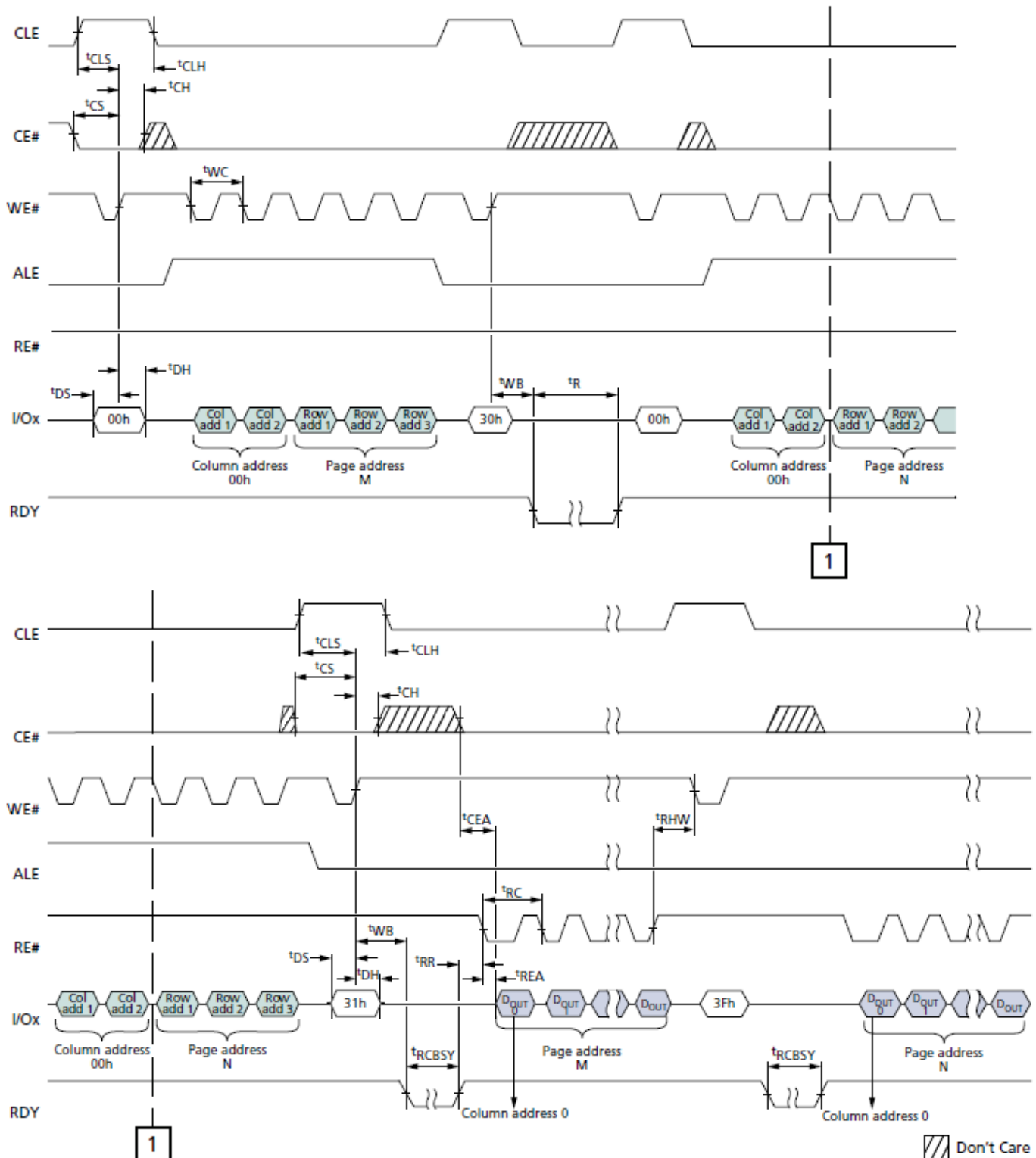
READ PAGE CACHE RANDOM
